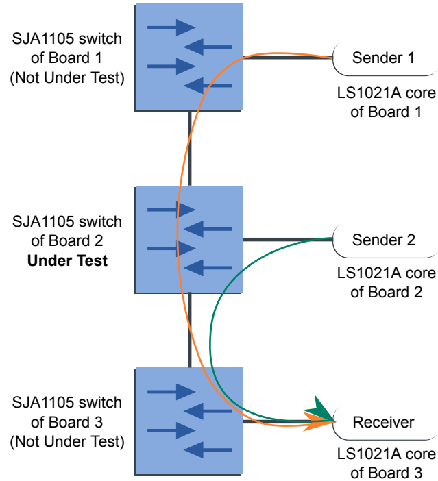
Figure 46. Connections of the three hosts and their roles as traffic senders/receivers
