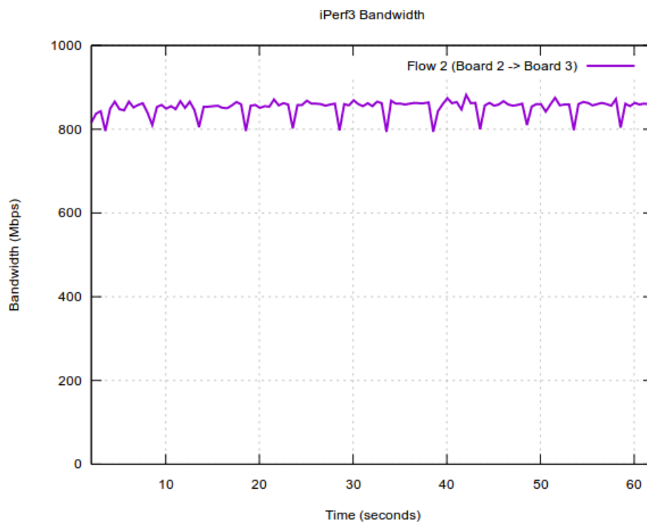
Figure 59. Policing configuration: Flow 2 run by its own
