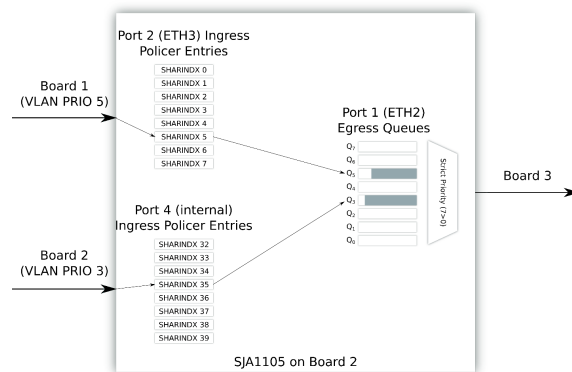
Figure 53. Prioritizing configuration
