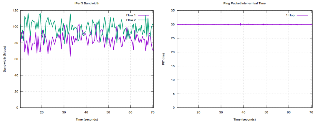
Figure 72. 1-hop ping with background traffic
