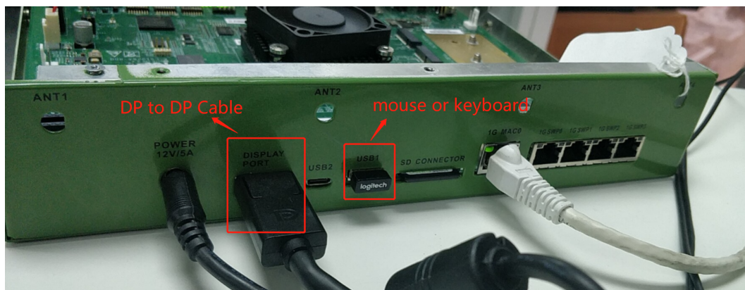
Figure 89. Hardware setup for QT
