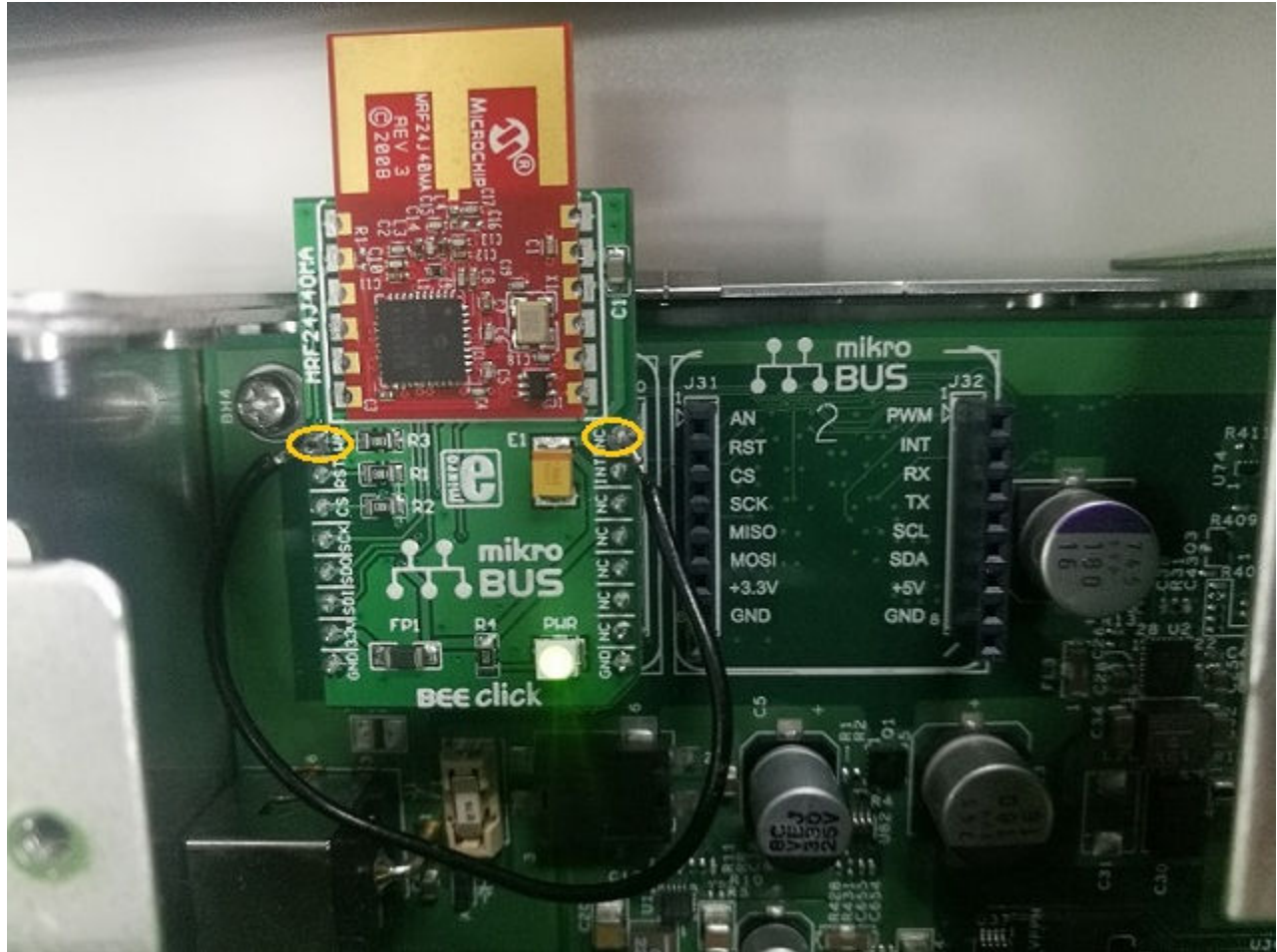
Figure 87. BEE Click Board hardware setup
