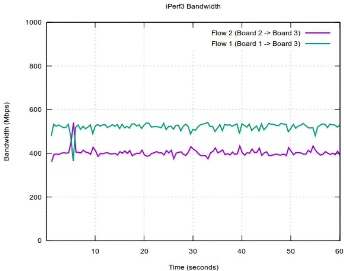
Figure 60. Policing configuration: both flows running at the same time
