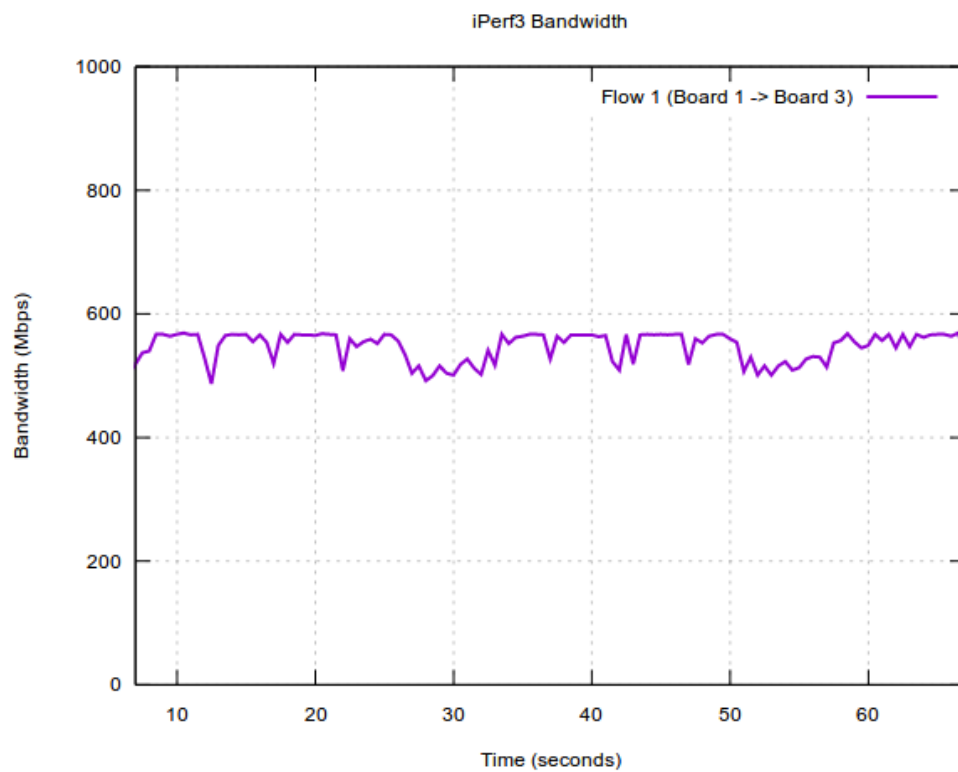
Figure 63. Scheduling configuration: Flow 1 run by its own
