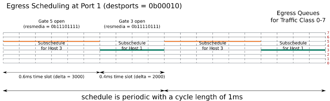
Figure 62. Time gating for Host 1 and Host 3, viewed on the time axis
