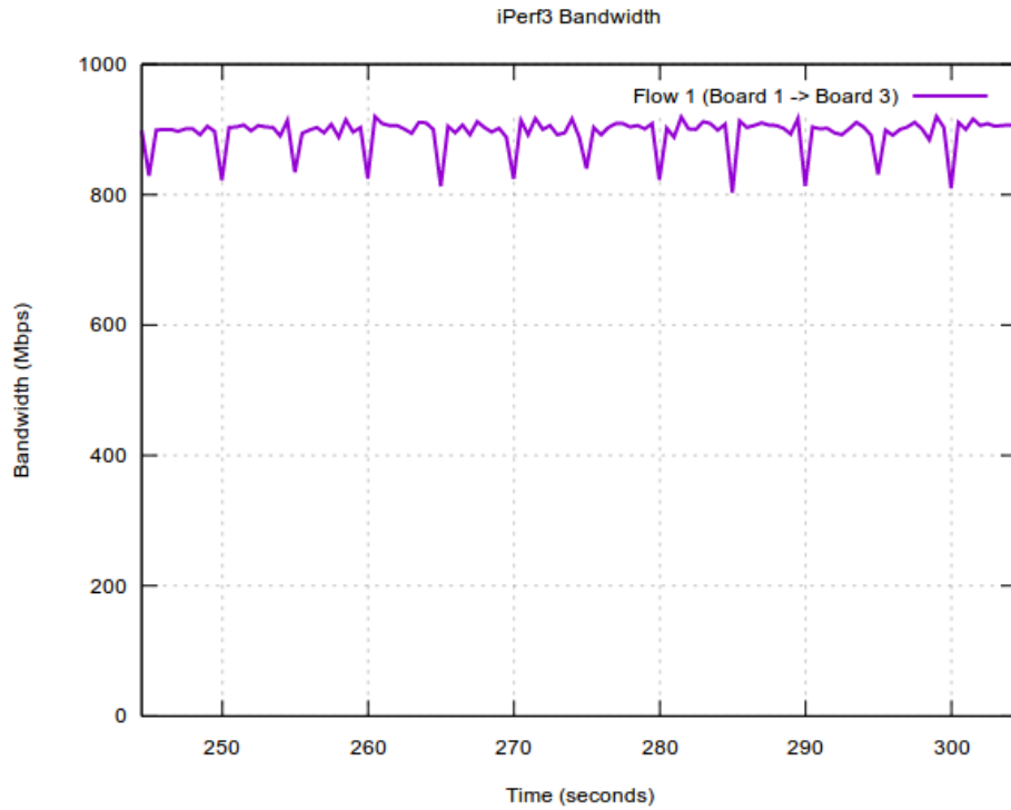
Figure 54. Prioritizing configuration: Flow 1 run by its own
