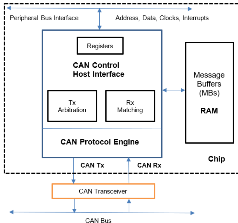
Figure 80. FlexCAN block diagram
