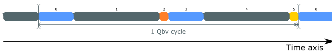
Figure 66. Qbv schedule
