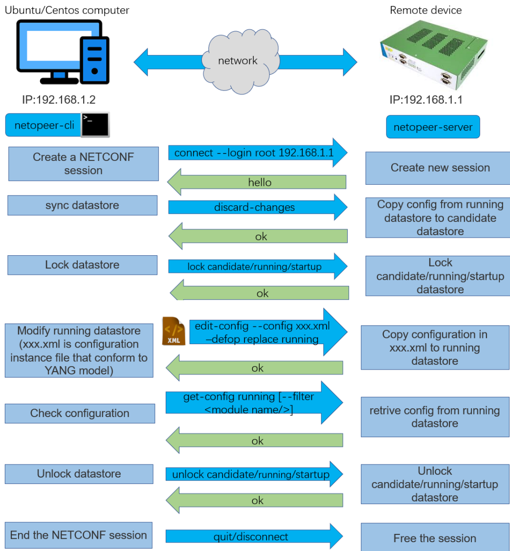
Figure 21. Steps to configure device via netopeer
