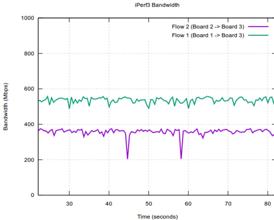
Figure 65. Both flows run at the same time
