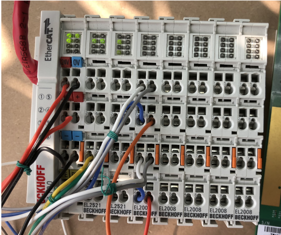
Figure 77. BECKHOFF EL2008
