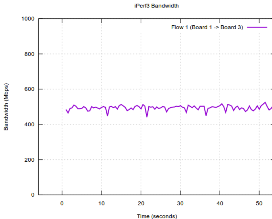
Figure 58. Policing configuration: Flow 1 run by its own
