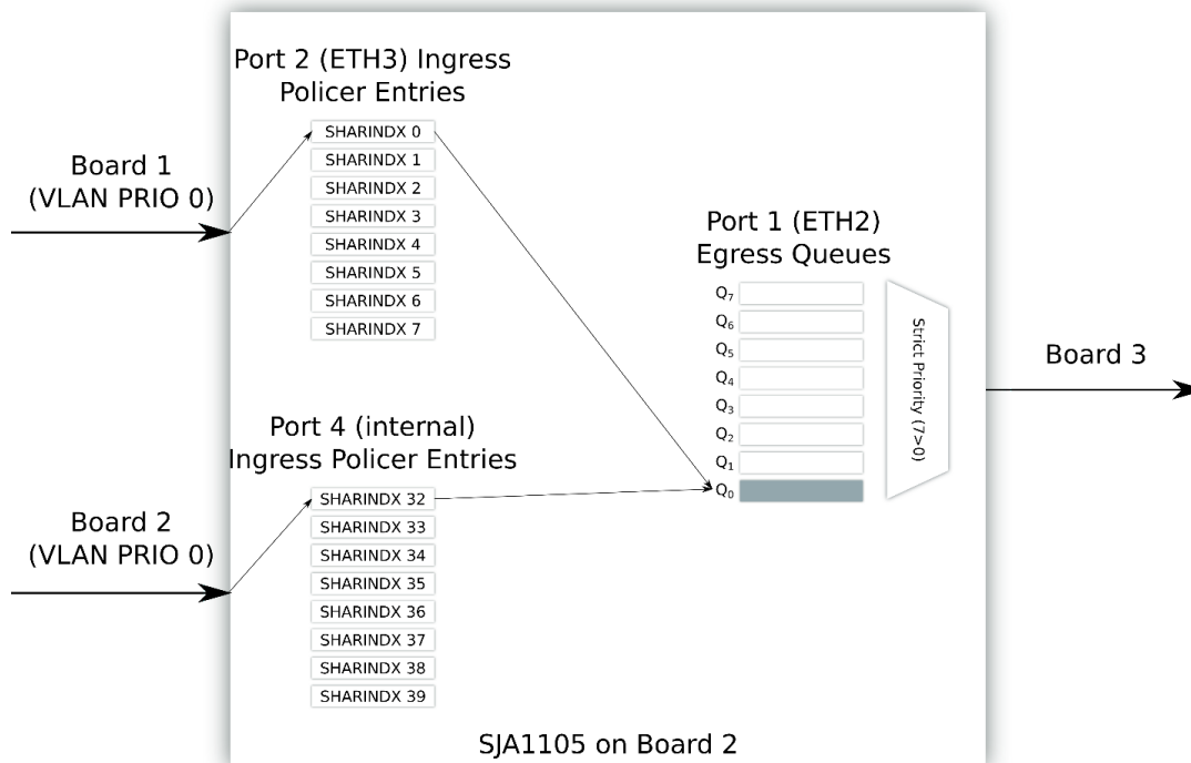
Figure 49. Queuing diagram
