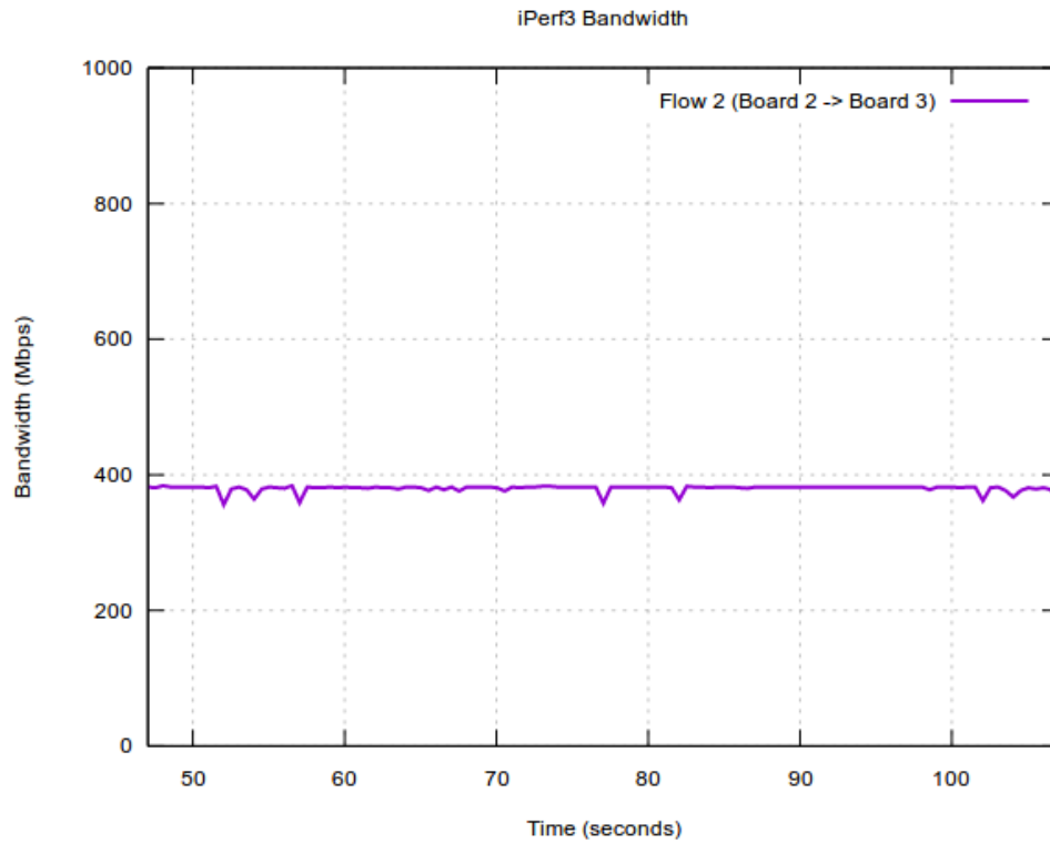
Figure 64. Scheduling configuration: Flow 2 run by its own
