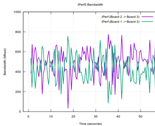
Figure 52. Standard configuration: Both flows run at the same time
