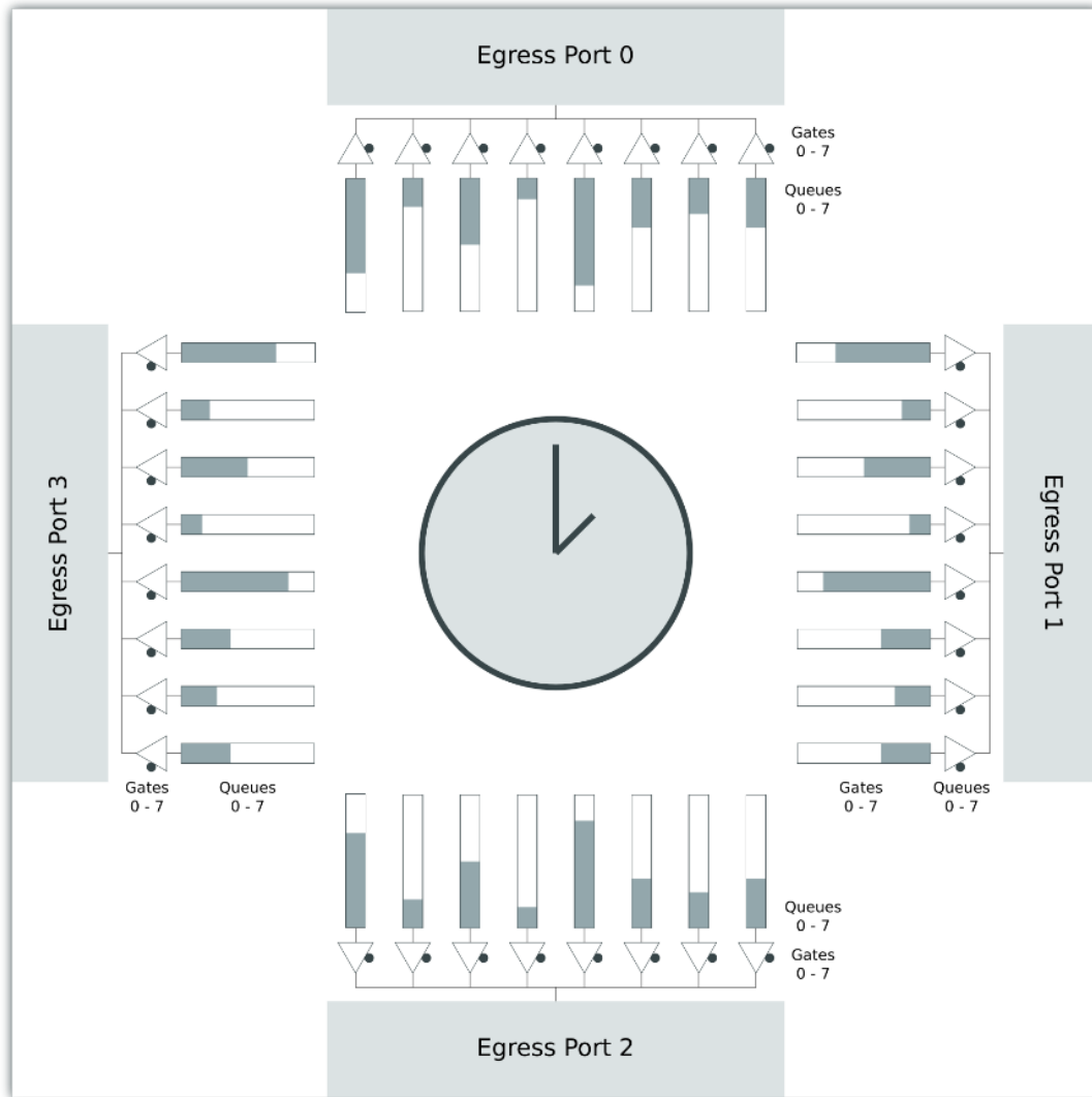
Figure 61. Structure of the Time Aware Scheduler
