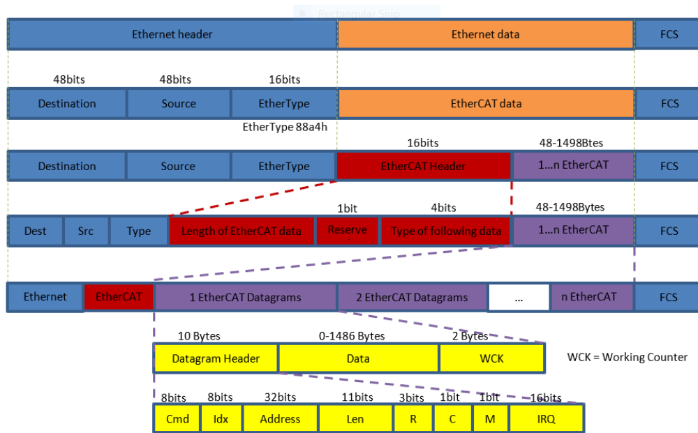
Figure 75. EtherCAT frame structure
