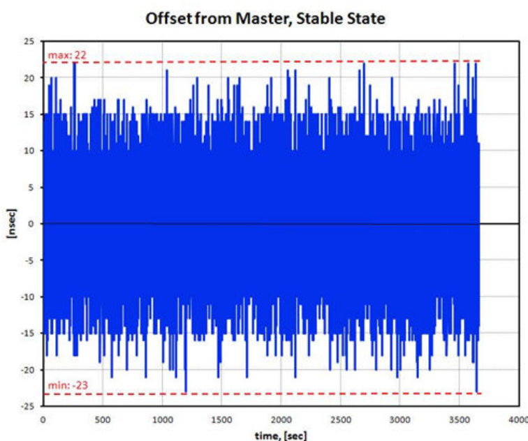
Figure 9. Offset from master in stable state
