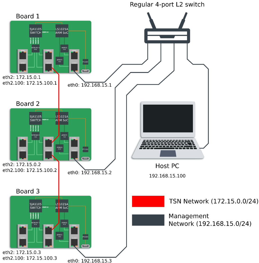
Figure 39. Topology of the demo network
