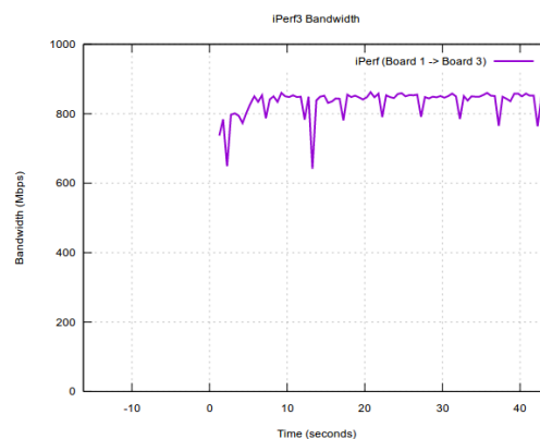
Figure 50. Standard configuration: Flow 1 run by its own
