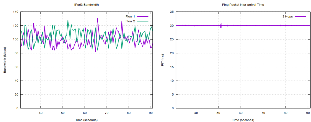
Figure 73. 3-hop ping with background traffic
