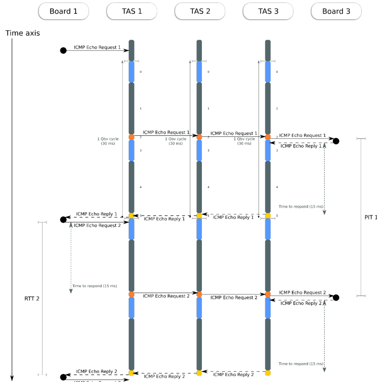
Figure 68. Timeslots in the 3 hop scenario
