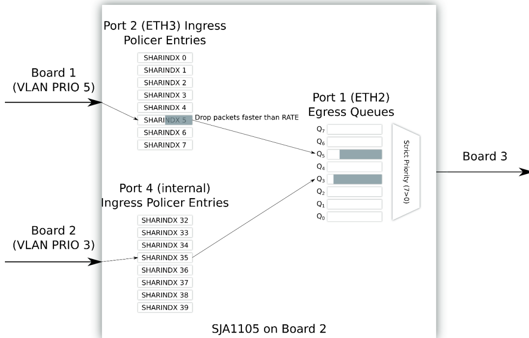
Figure 57. Queuing diagram for policing configuration
