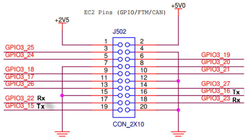
Figure 85. Hardware diagram for the FlexCan demo
