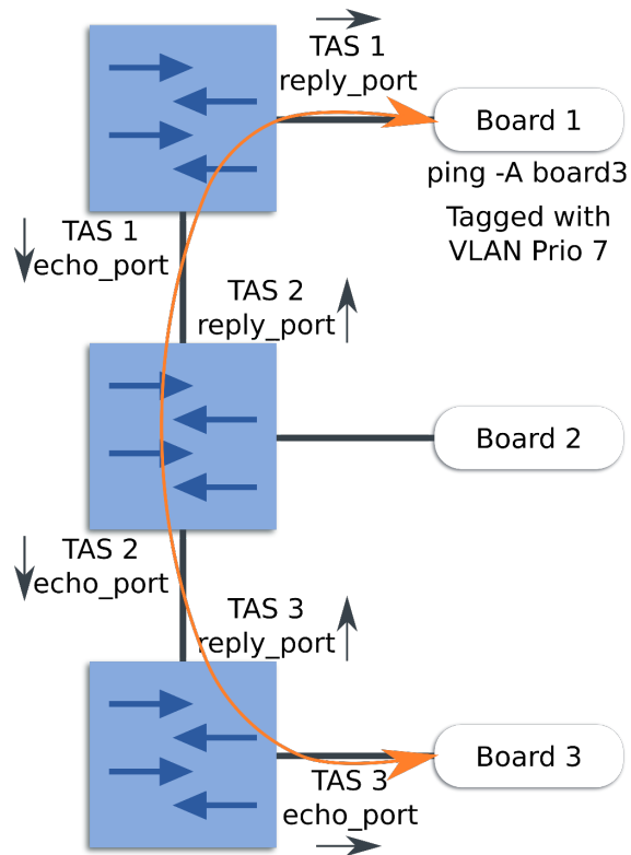
Figure 67. 3-hop scenario
