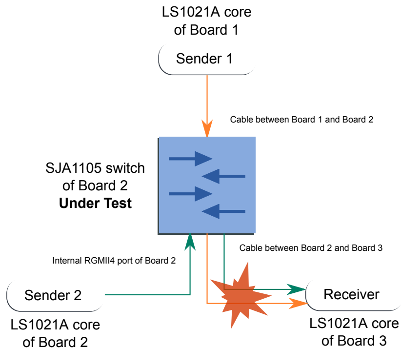
Figure 47. Simplified traffic flows for the rate limiting use case
