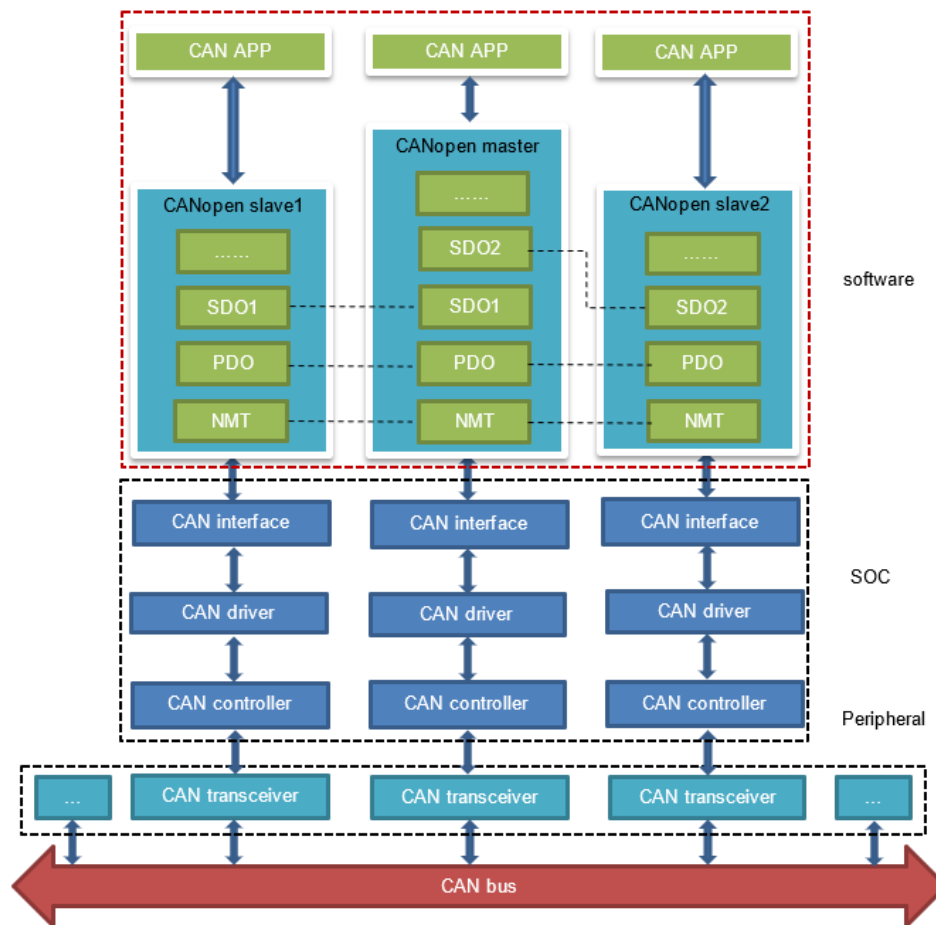
Figure 84. CANopen architecture
