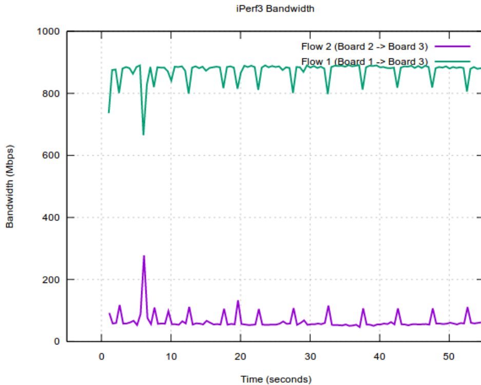
Figure 56. Prioritizing configuration: both flows run at the same time
