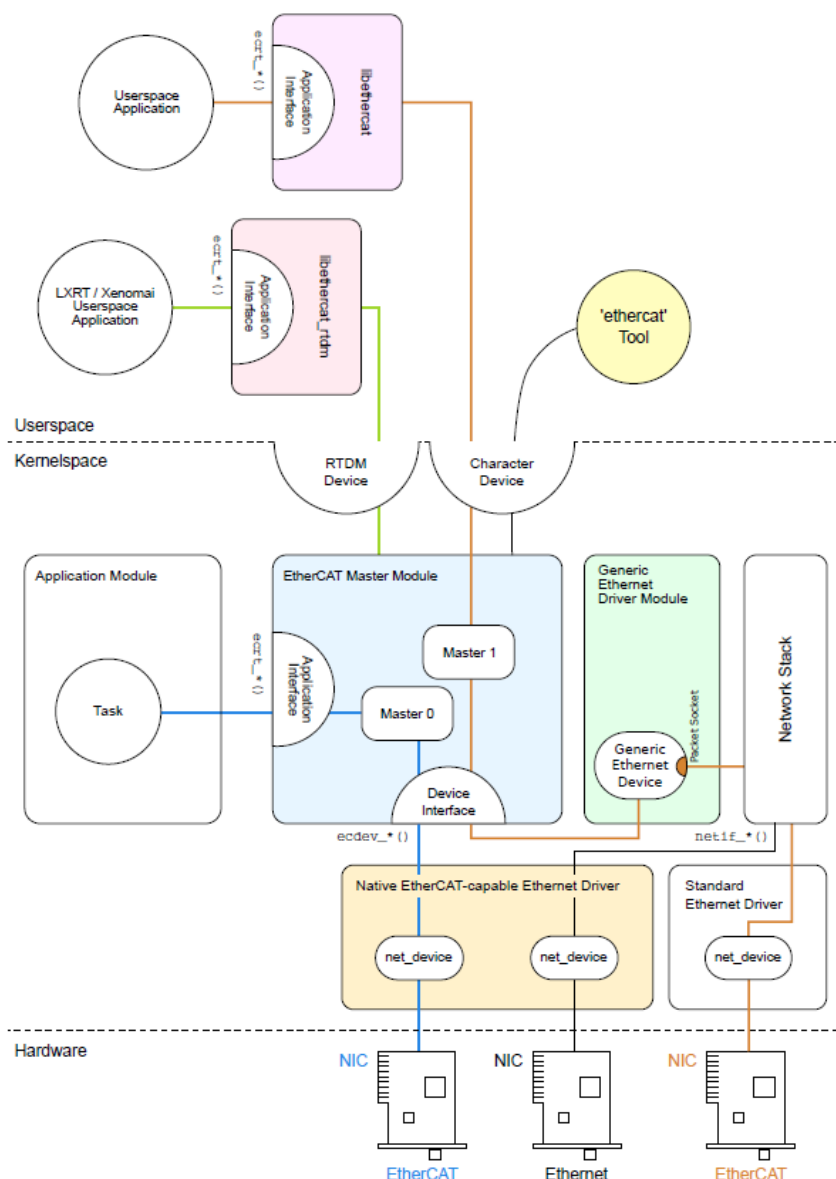
Figure 74. IGH EtherCAT master architecture
