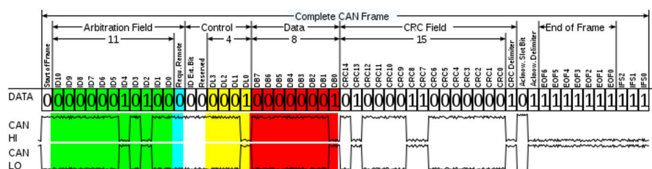
Figure 75. Base frame format
