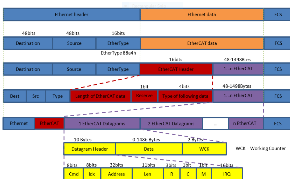
Figure 68. EtherCAT frame structure
