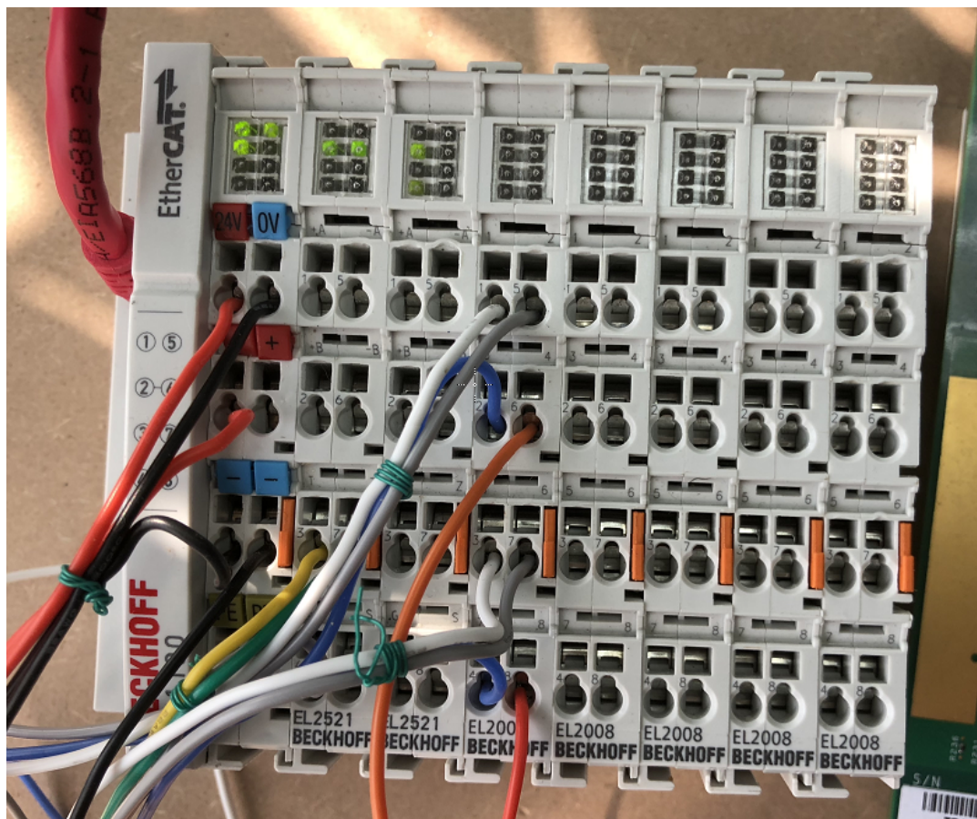
Figure 70. BECKHOFF EL2008
