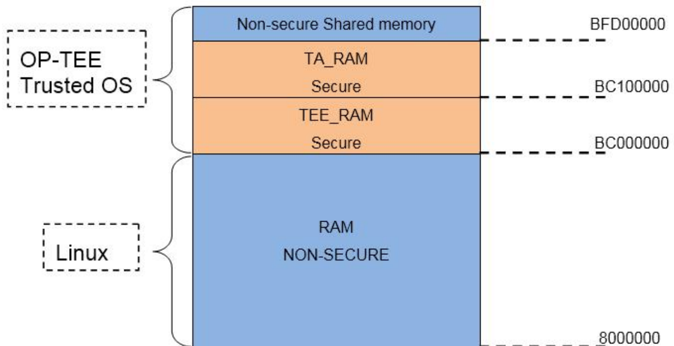
Figure 9. DDR memory map
