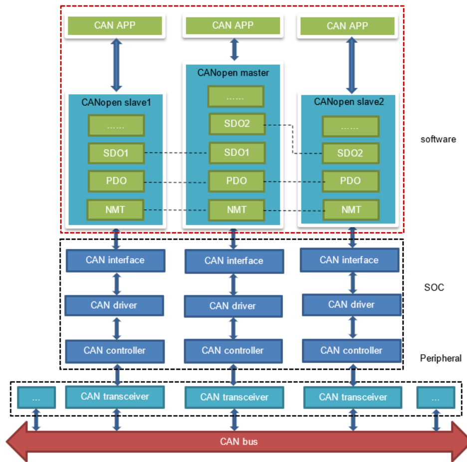
Figure 77. CANopen architecture
