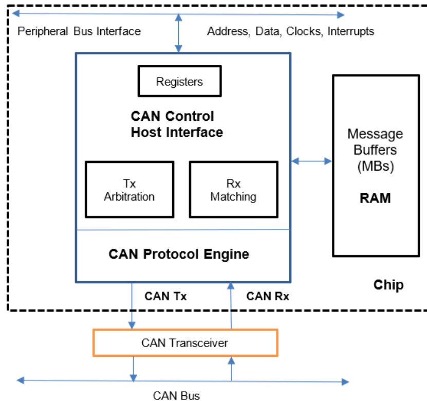
Figure 73. FlexCAN block diagram
