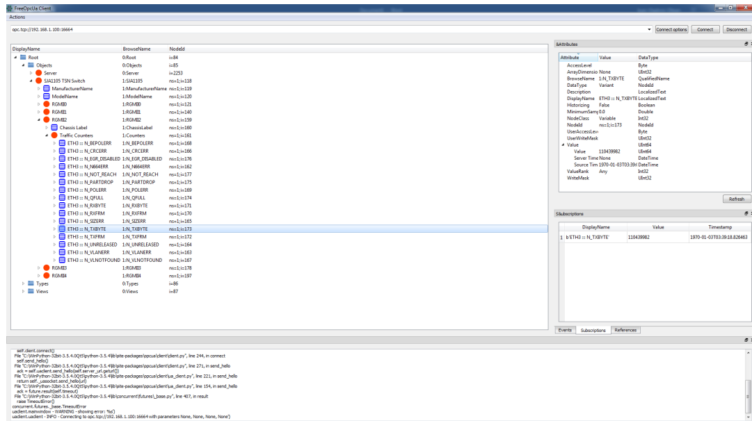
Figure 20. Subscribing to data changes of the ETH3 ::: N_TXBYTE node of the OPC-SJA1105 server
