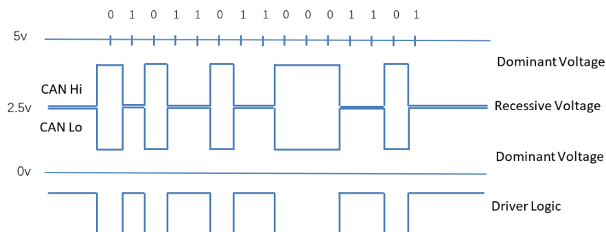
Figure 74. High speed CAN signaling
