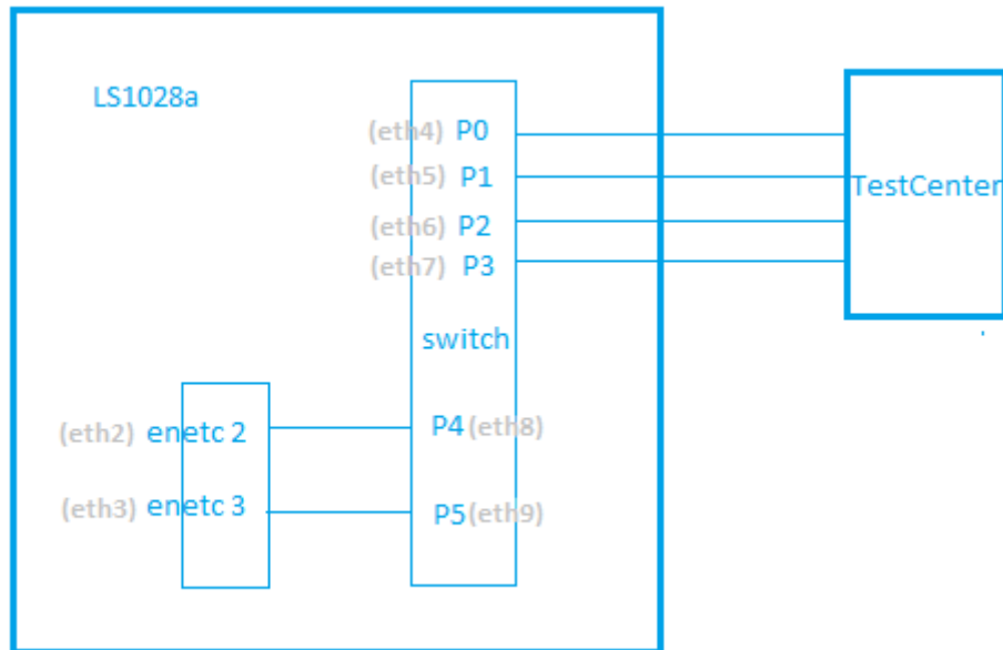
Figure 61. TSN switch configuration
