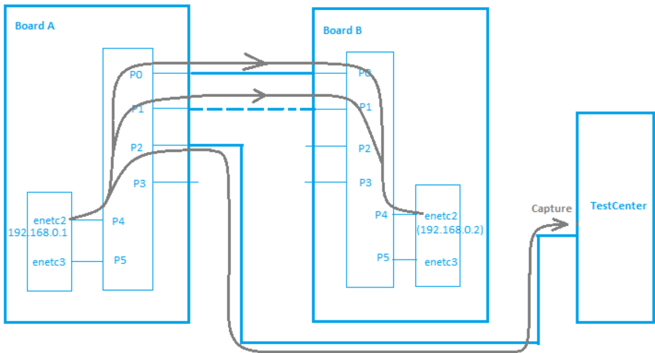
Figure 66. Seamless redundancy test
