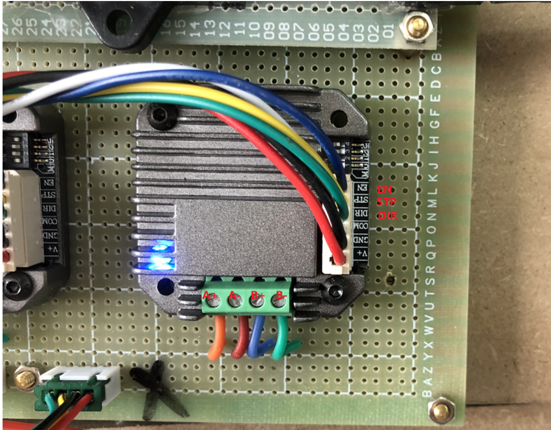
Figure 71. Stepper motor driver
