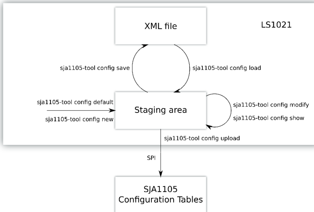
Figure 27. State machine view of the sja1105-tool commands and configuration formats
