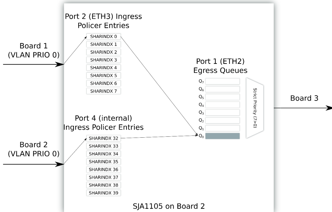
Figure 32. Queuing diagram
