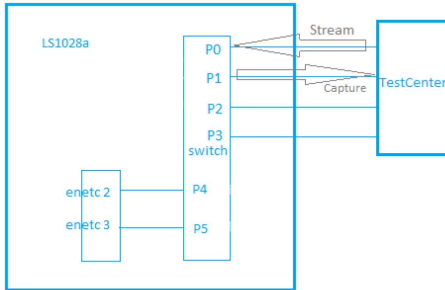
Figure 62. Qbv test
