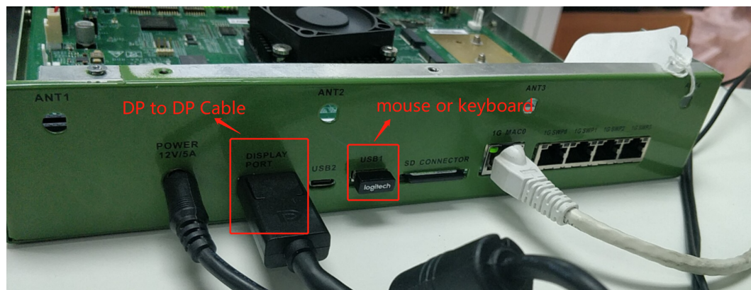
Figure 80. Hardware setup for QT
