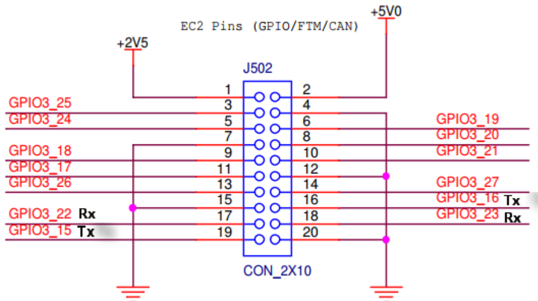
Figure 78. Hardware diagram for the FlexCan demo
