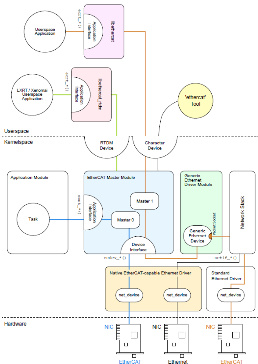
Figure 67. IGH EtherCAT master architecture
