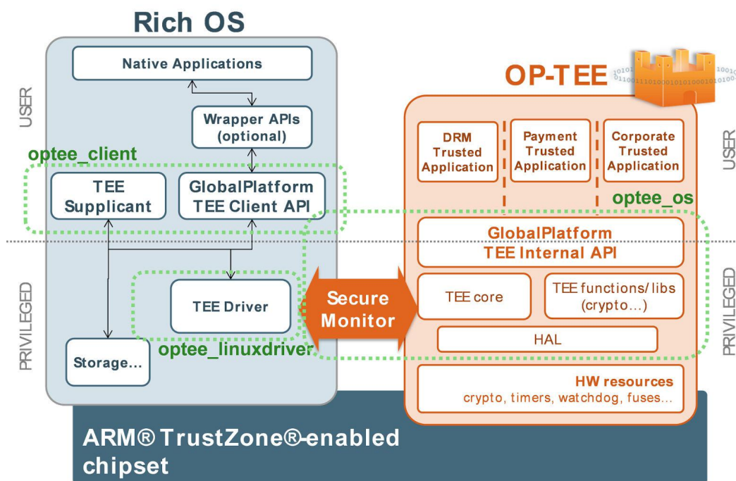
Figure 7. Architecture of OP-TEE on an ARM TrustZone enabled SoC
