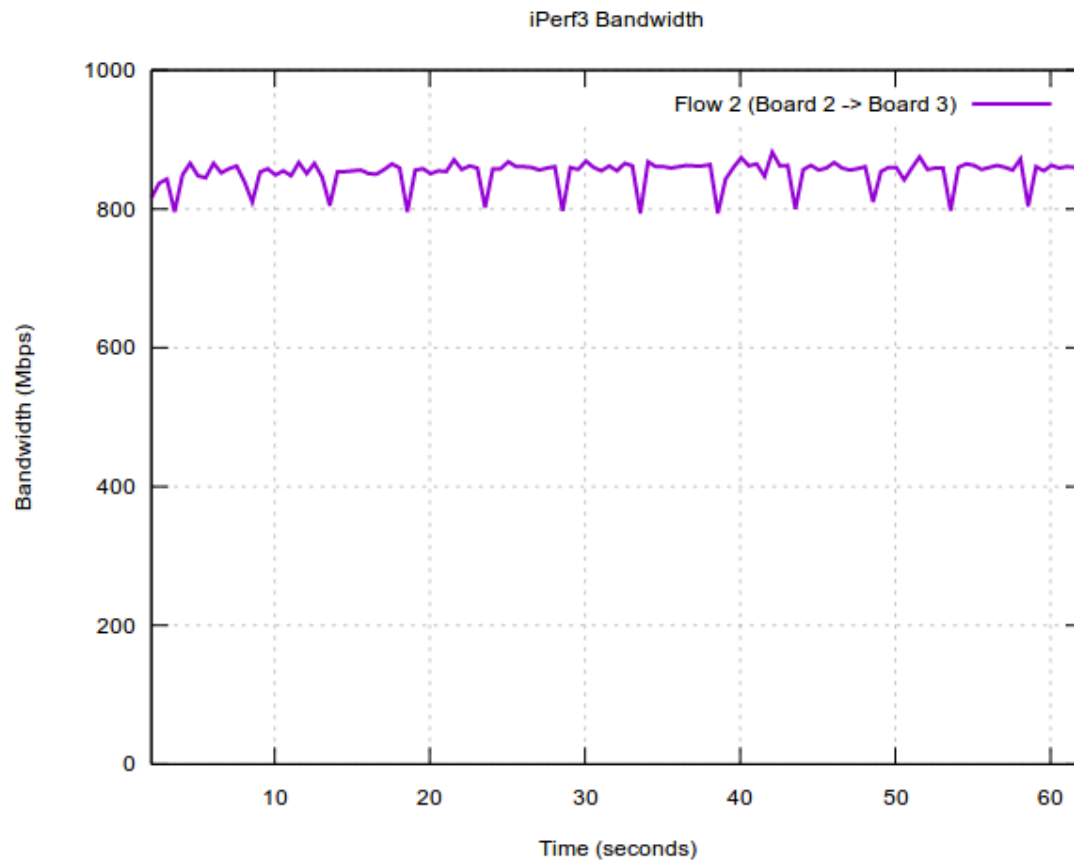
Figure 41. Policing configuration: Flow 2 run by its own
