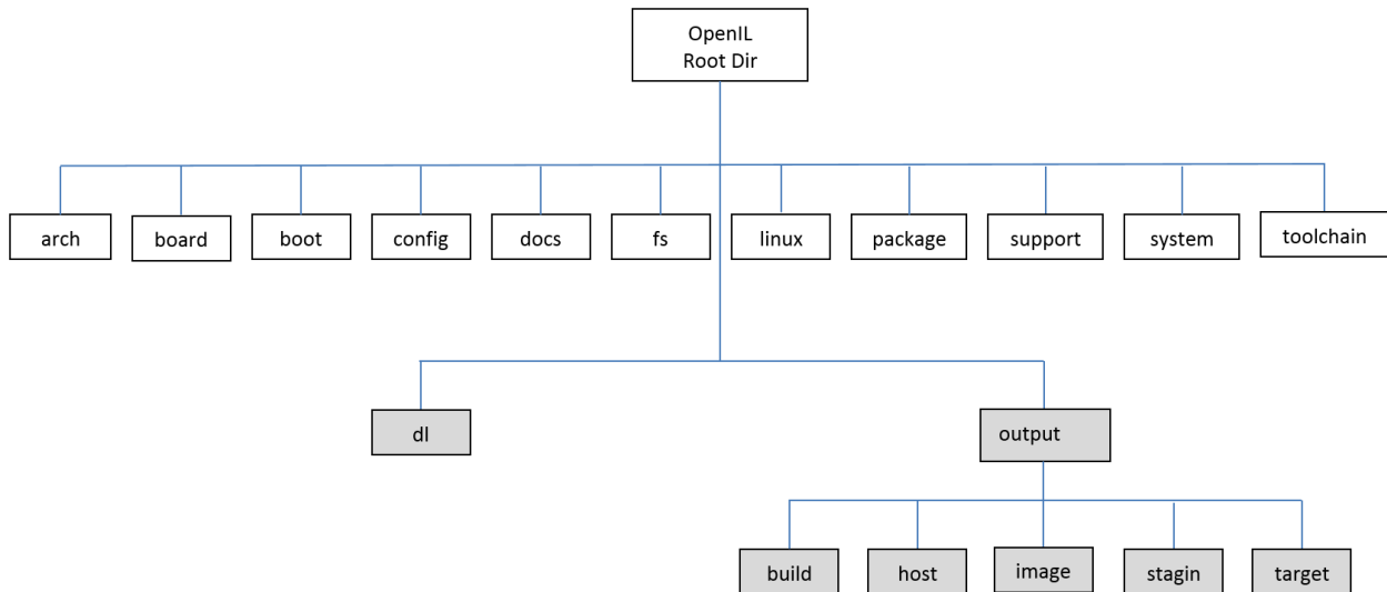
Figure 1. OpenIL structure
