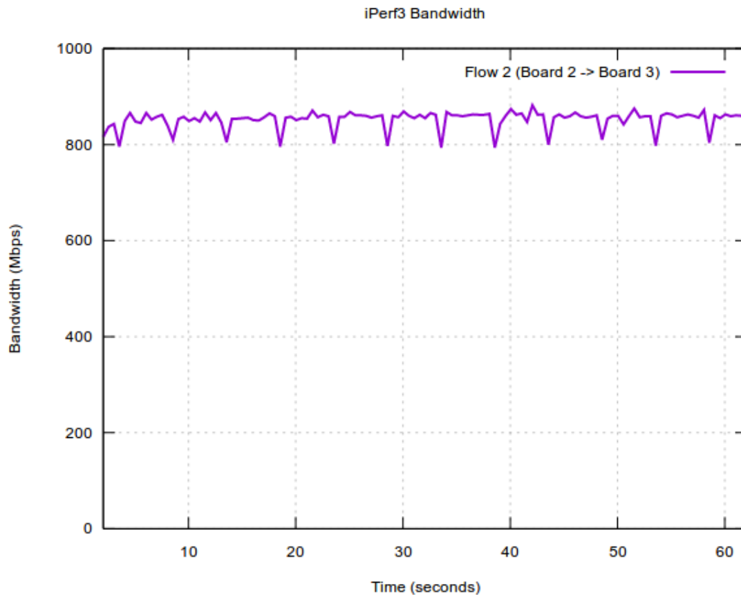
Figure 41. Policing configuration: Flow 2 run by its own
