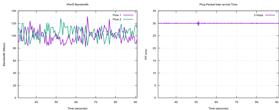
Figure 55. 3-hop ping with background traffic
