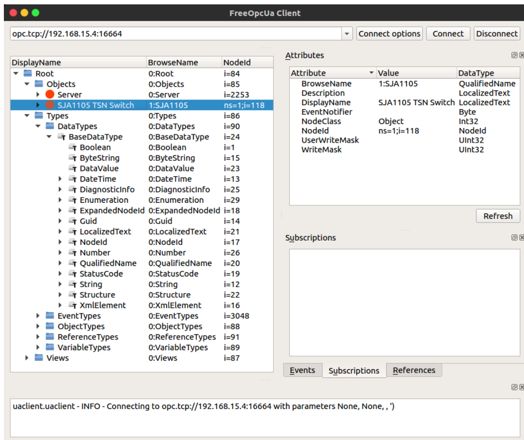
Figure 16. OPC UA address space
