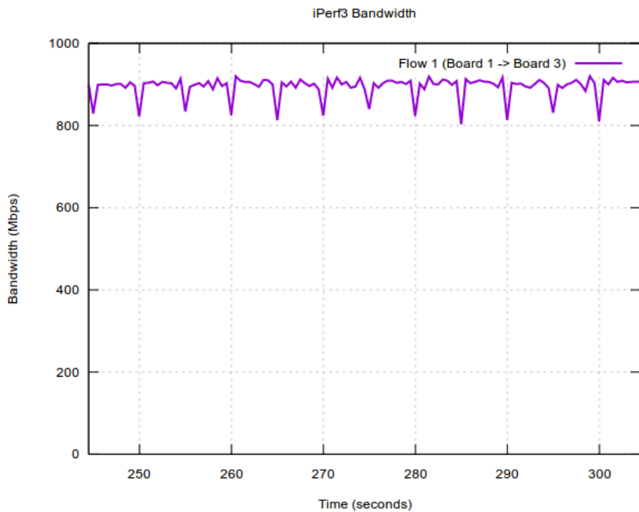
Figure 36. Prioritizing configuration: Flow 1 run by its own
