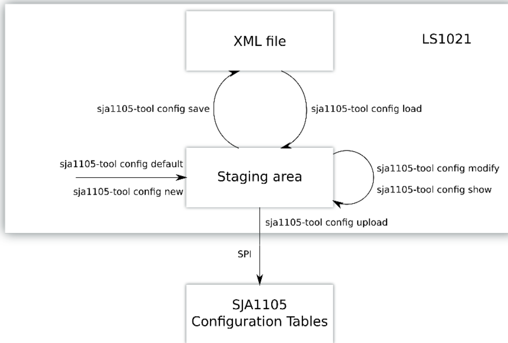
Figure 26. State machine view of the sja1105-tool commands and configuration formats
