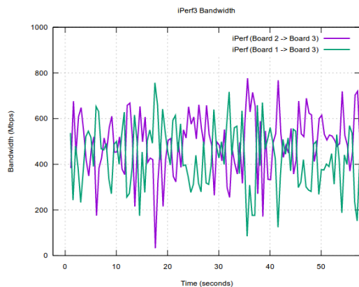
Figure 34. Standard configuration: Both flows run at the same time
