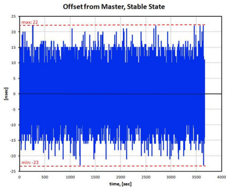
Figure 6. Offset from master in stable state
