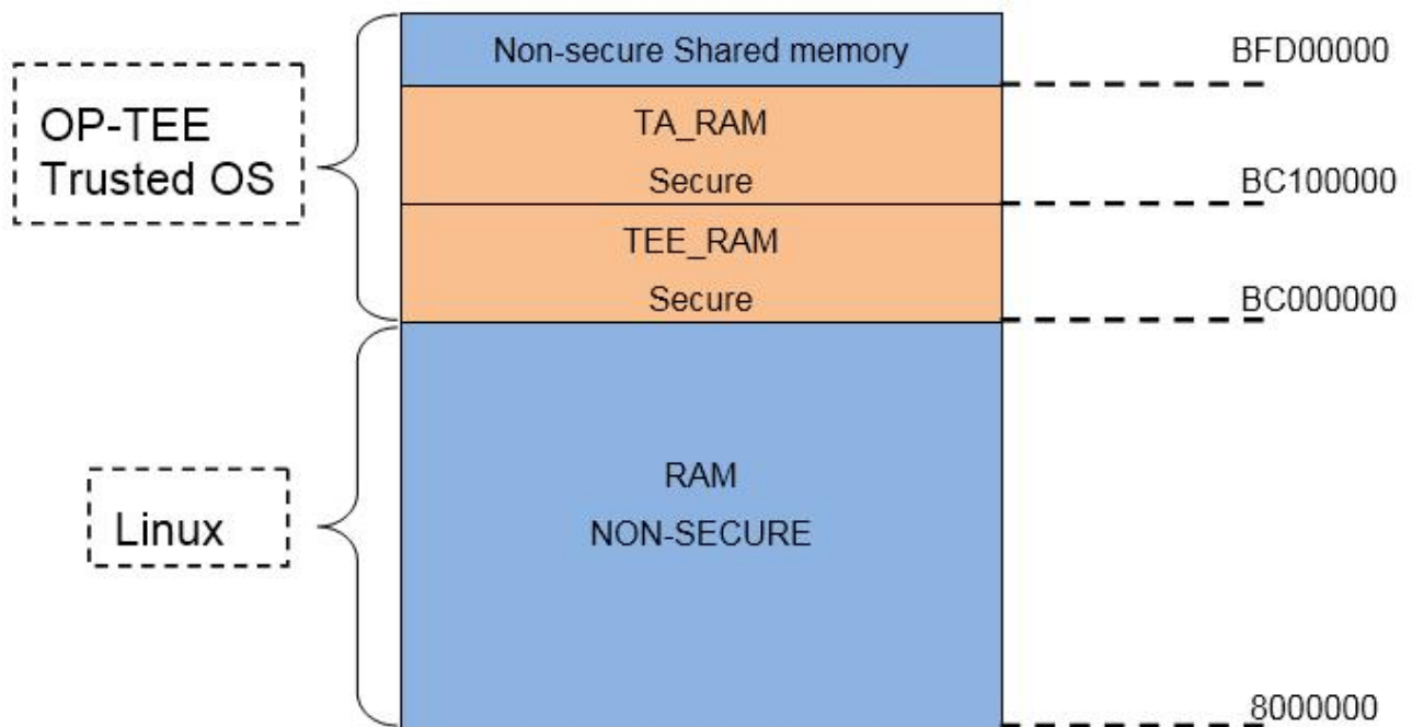
Figure 8. DDR memory map
