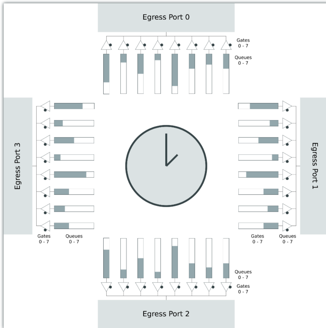
Figure 43. Structure of the Time Aware Scheduler
