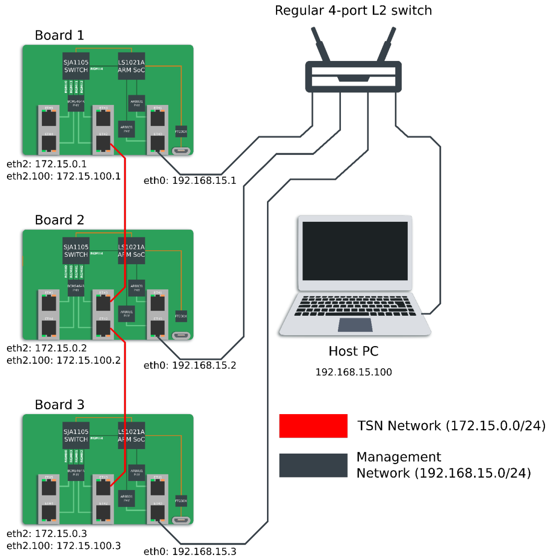
Figure 21. Topology of the demo network
