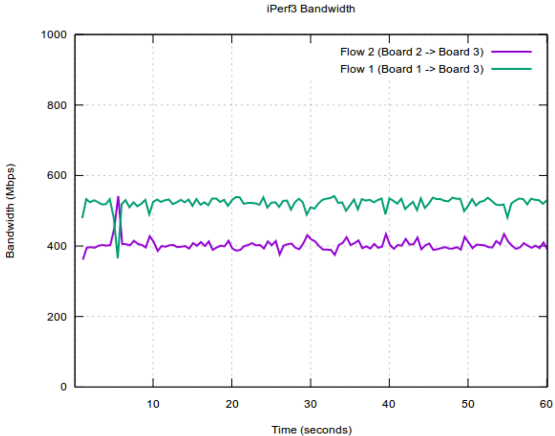
Figure 42. Policing configuration: both flows running at the same time
