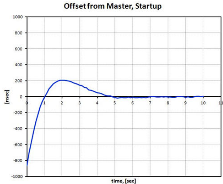
Figure 5. Offset from master in start up state
