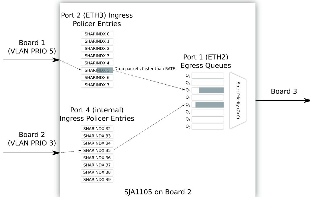
Figure 39. Queuing diagram for policing configuration
