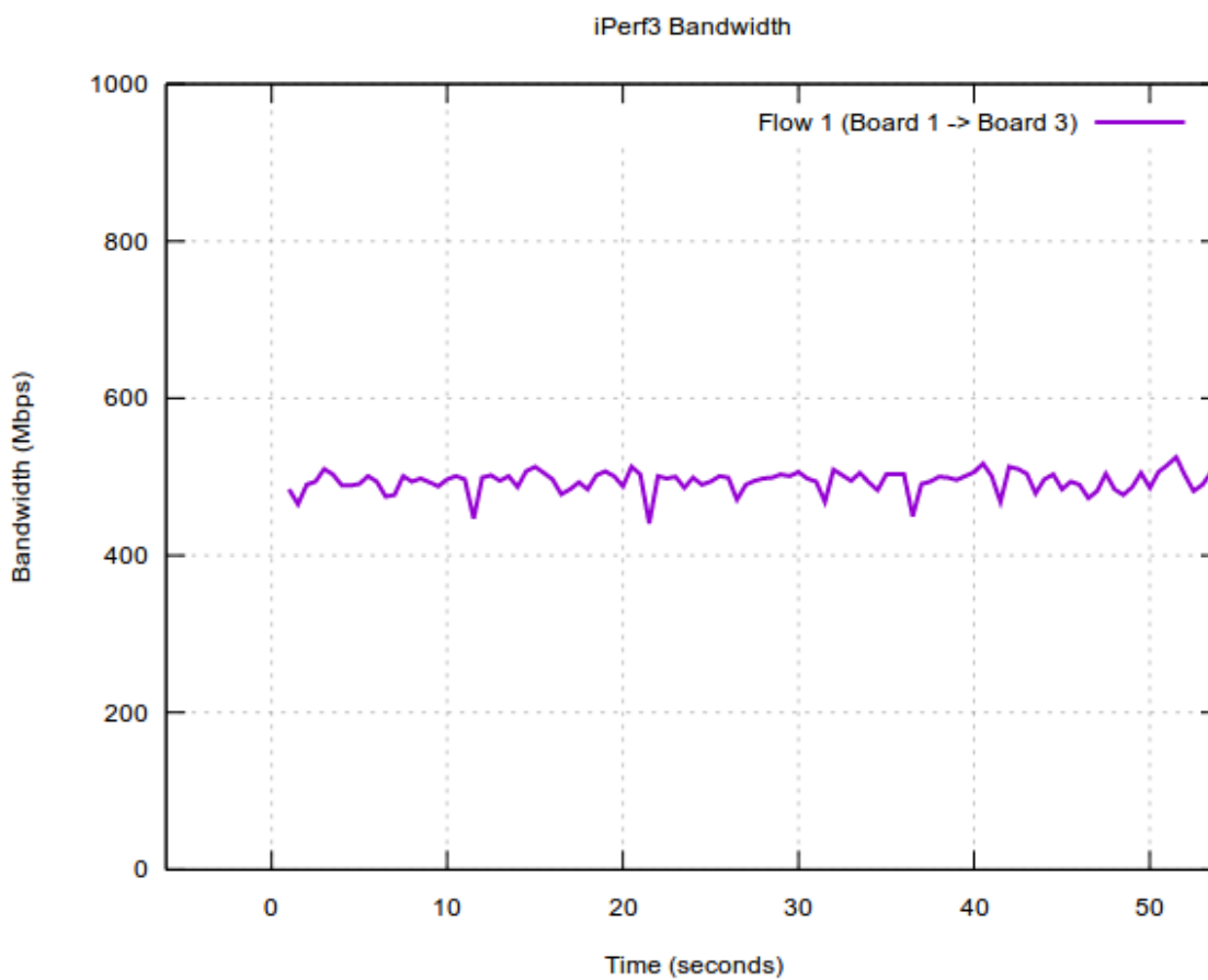
Figure 40. Policing configuration: Flow 1 run by its own
