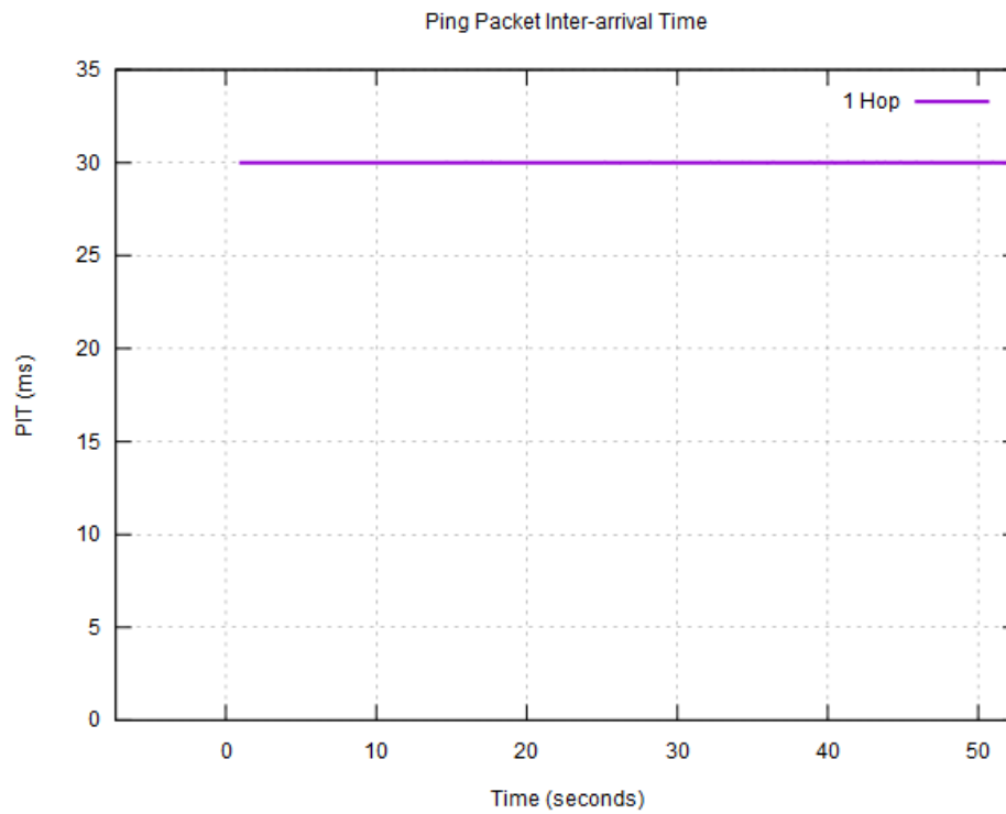
Figure 52. 1-hop flow
