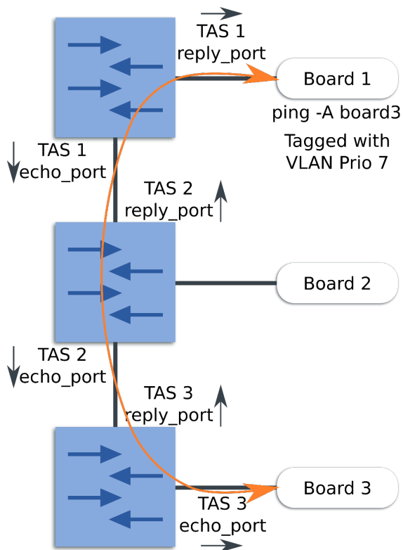
Figure 49. 3-hop scenario
