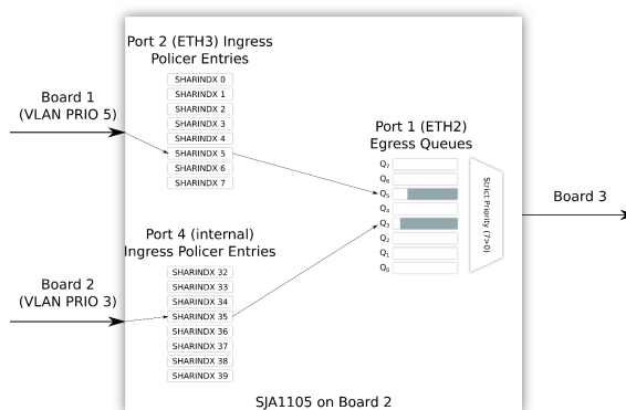
Figure 35. Prioritizing configuration
