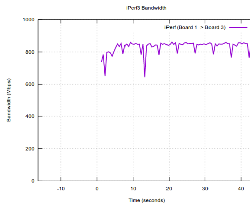
Figure 32. Standard configuration: Flow 1 run by its own
