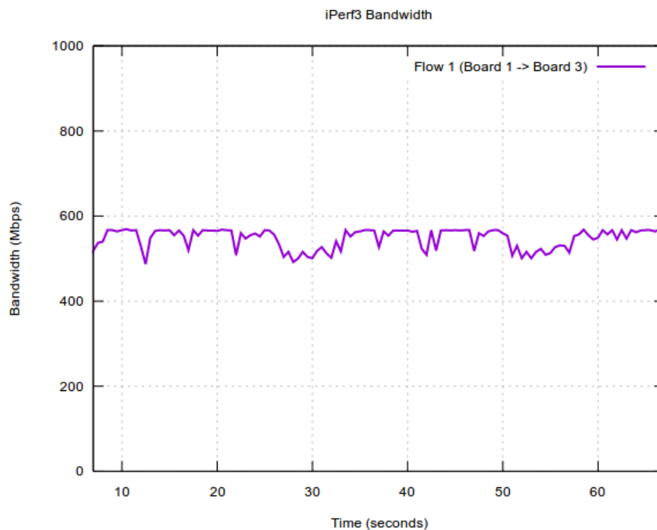
Figure 45. Scheduling configuration: Flow 1 run by its own
