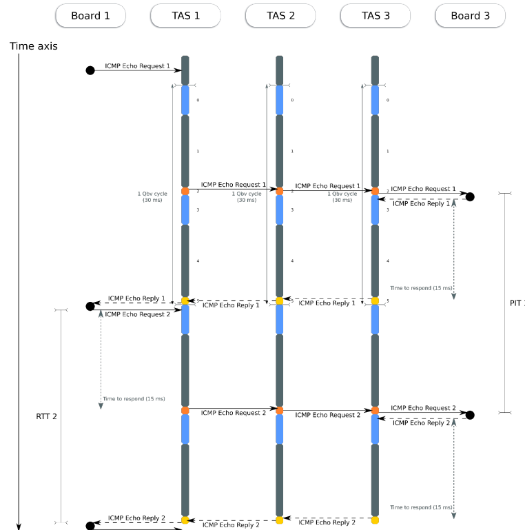
Figure 50. Timeslots in the 3 hop scenario
