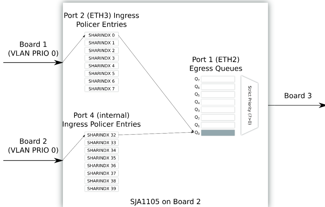
Figure 31. Queuing diagram
