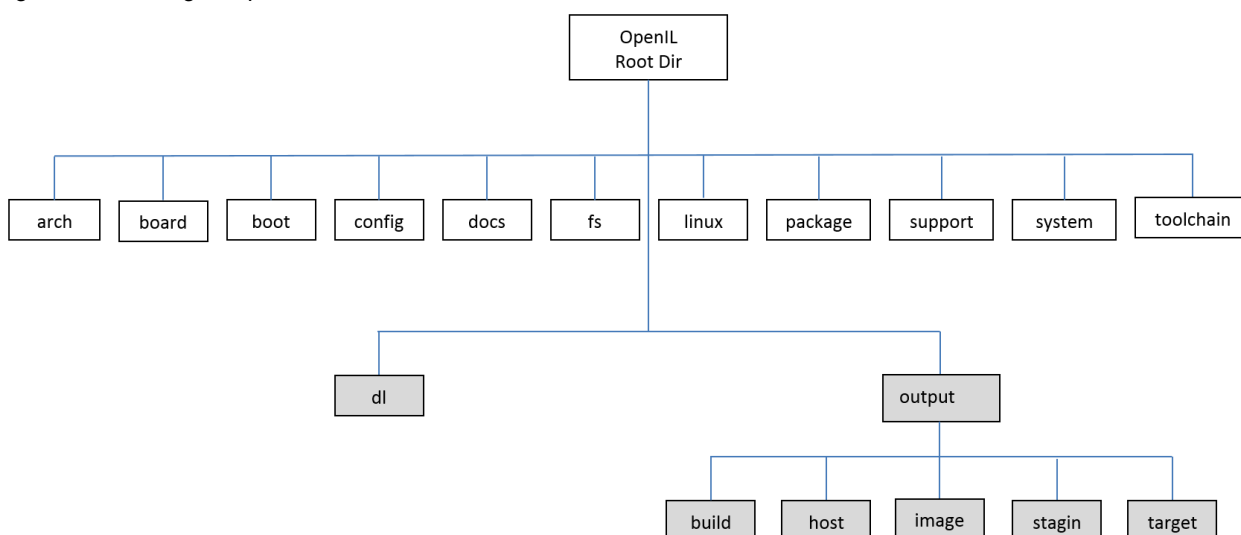
Figure 1. OpenIL structure
