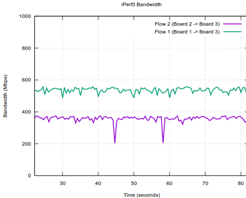
Figure 47. Both flows run at the same time
