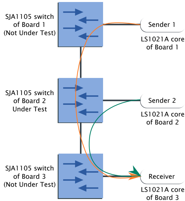
Figure 28. Connections of the three hosts and their roles as traffic senders/receivers
