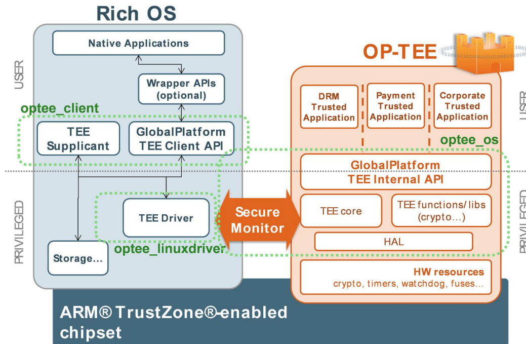
Figure 7. Architecture of OP-TEE on an ARM TrustZone enabled SoC
