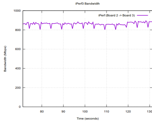
Figure 33. Standard configuration: Flow 2 run by its own
