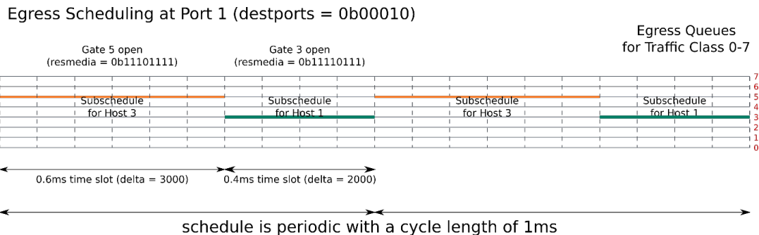
Figure 44. Time gating for Host 1 and Host 3, viewed on the time axis
