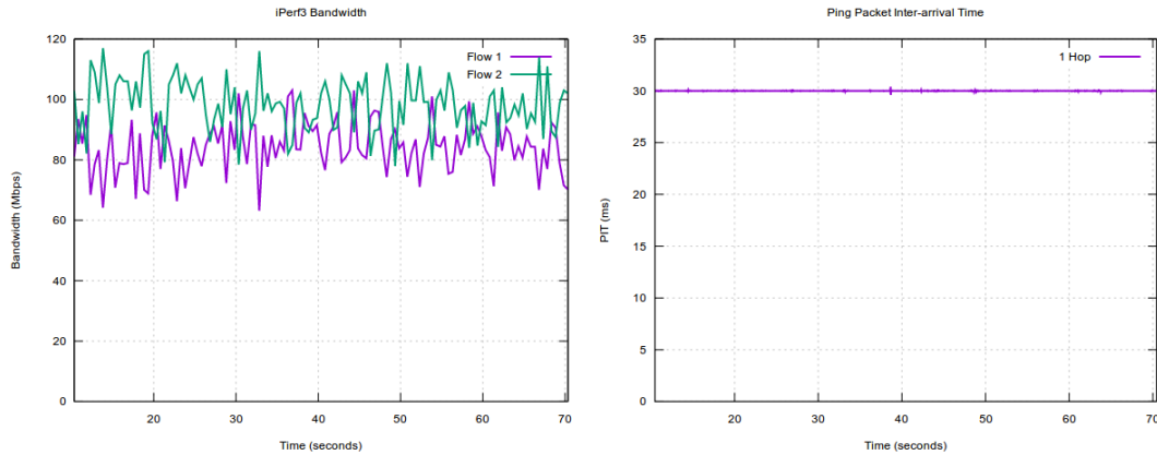
Figure 54. 1-hop ping with background traffic
