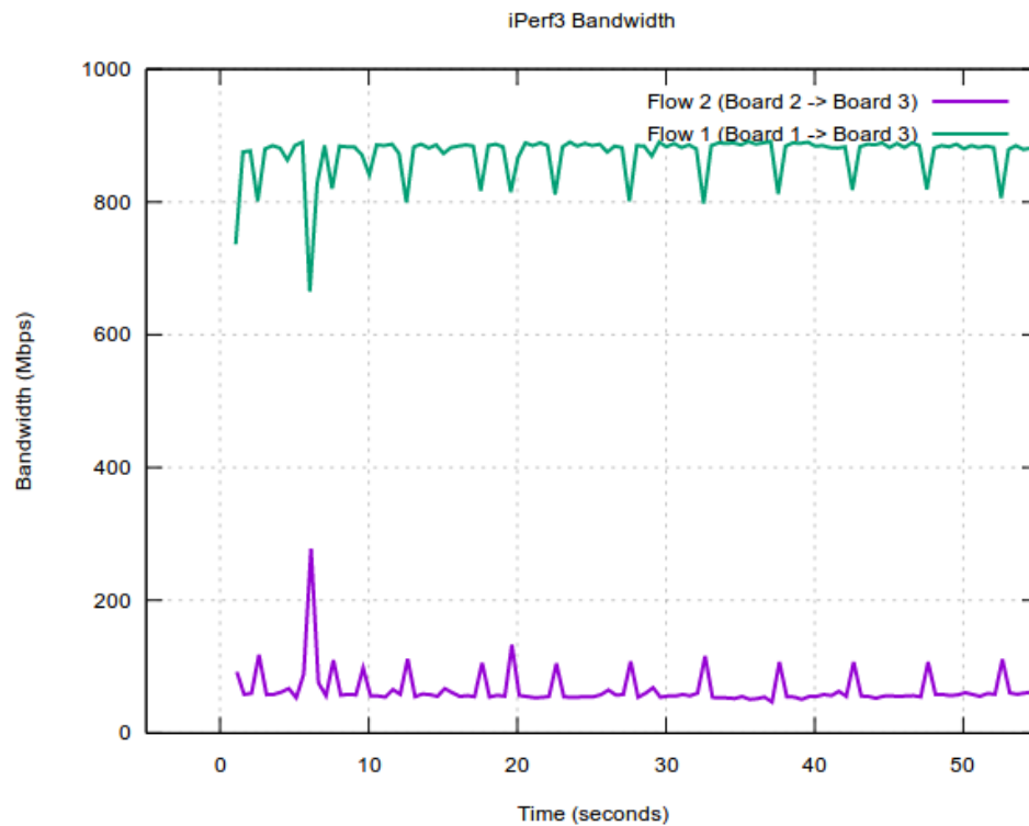
Figure 38. Prioritizing configuration: both flows run at the same time
