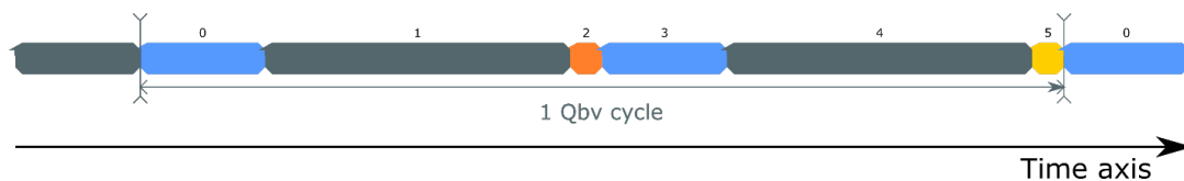
Figure 48. Qbv schedule
