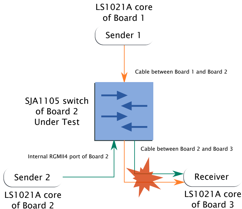
Figure 29. Simplified traffic flows for the rate limiting use case
