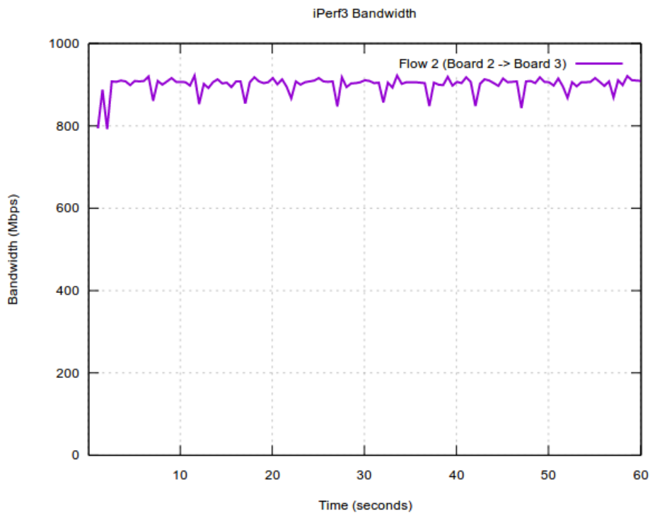
Figure 37. Prioritizing configuration: Flow 2 run by its own
