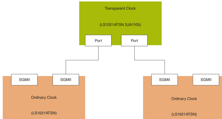
Figure 4. LS1021ATSN TC synchronization
